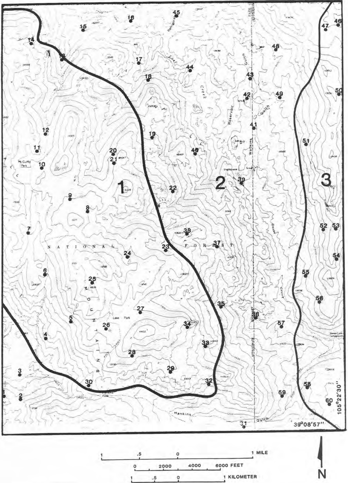
Figure 6. Geologic map.
